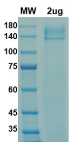
SDS-PAGE Image
