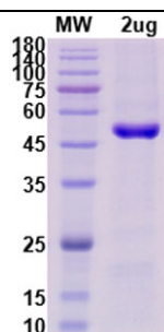
SDS-PAGE Image
